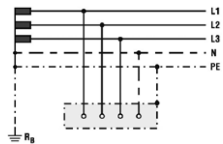
TN-S system
