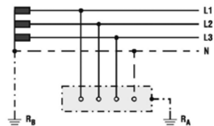
TT system
